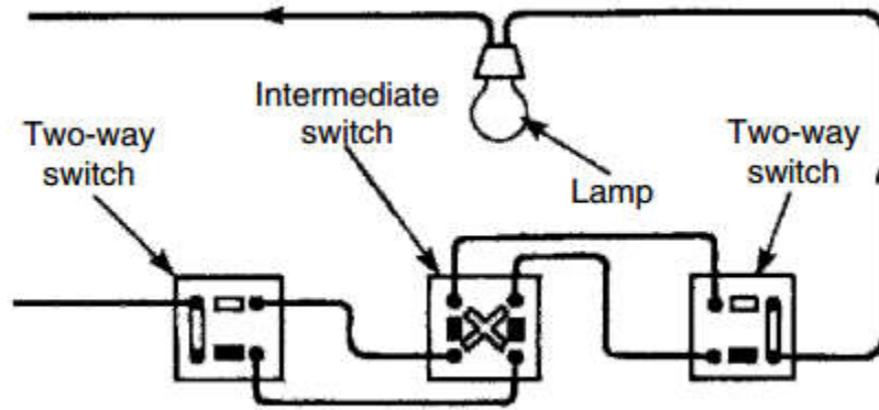
FIGURE 6.5: Two-way switching with one intermediate switch
