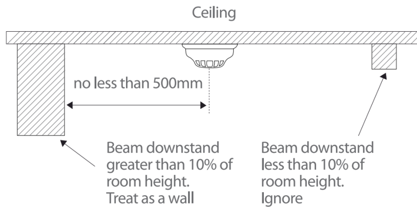
FIGURE 7.3: Spacing under obstructions.
