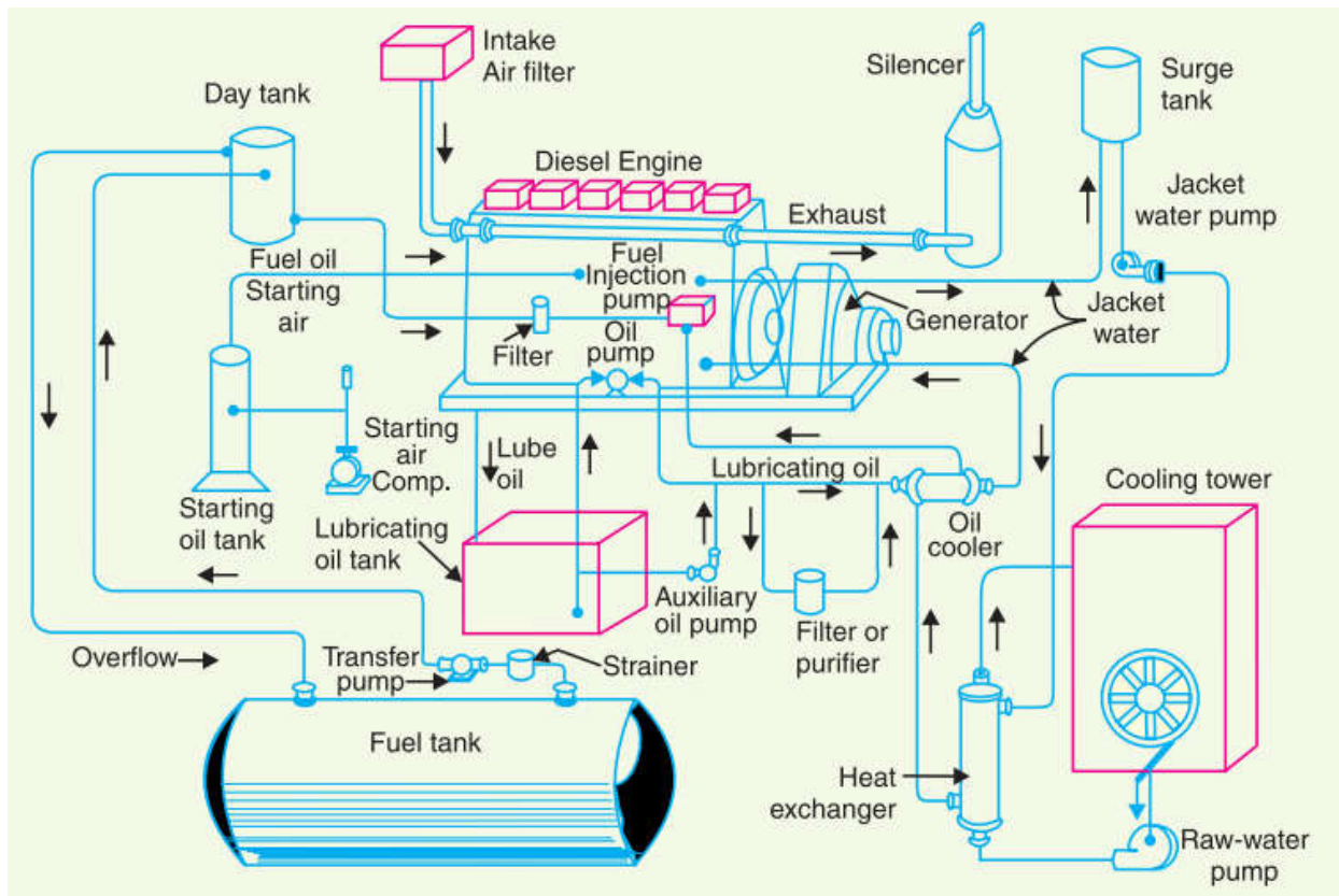
Schematic Arrangement of a Diesel Power Station
