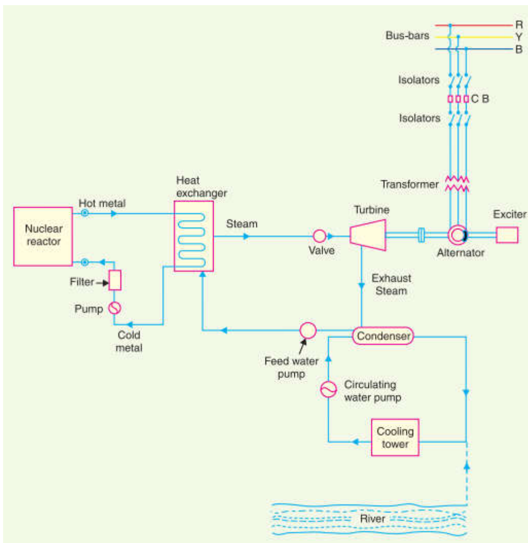
Schematic Arrangement of a Nuclear Power Station
