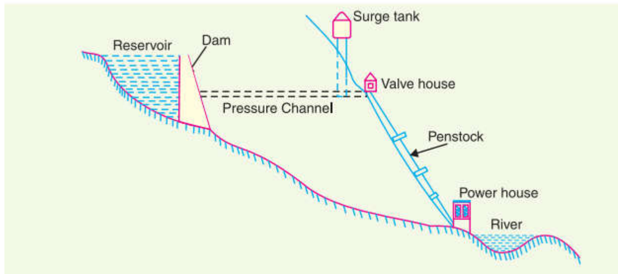
Schematic Arrangement of a Hydro-electric plant
