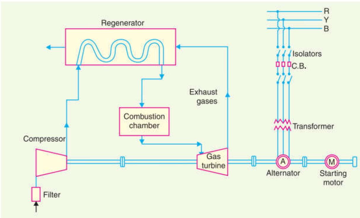
Schematic arrangement of gas turbine power
