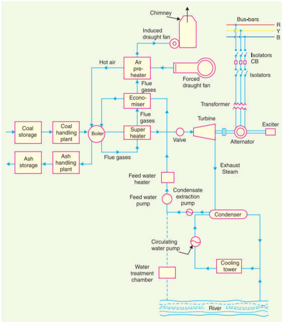
Schematic arrangement of a steam power plant
